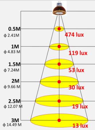
LUXEON 3535 2D- 135D WW
