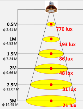
LUXEON 3535 2D- 135D TW
